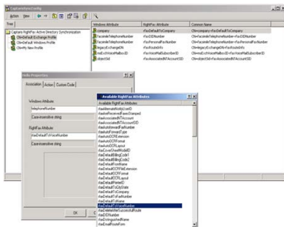
Figure 4. RightFax Active Directory Synchronization is available as a Microsoft Management Console (MMC) Snap-in.
